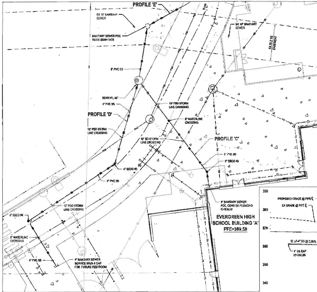
SANITARY SEWER PLAN 'C' and 'D' SCALE: 1" = 10'
